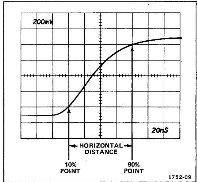
Figure 2-8. Measuring risetime.
